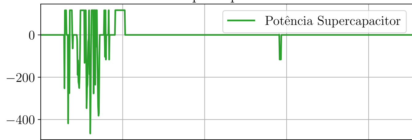
Supercapacitor
